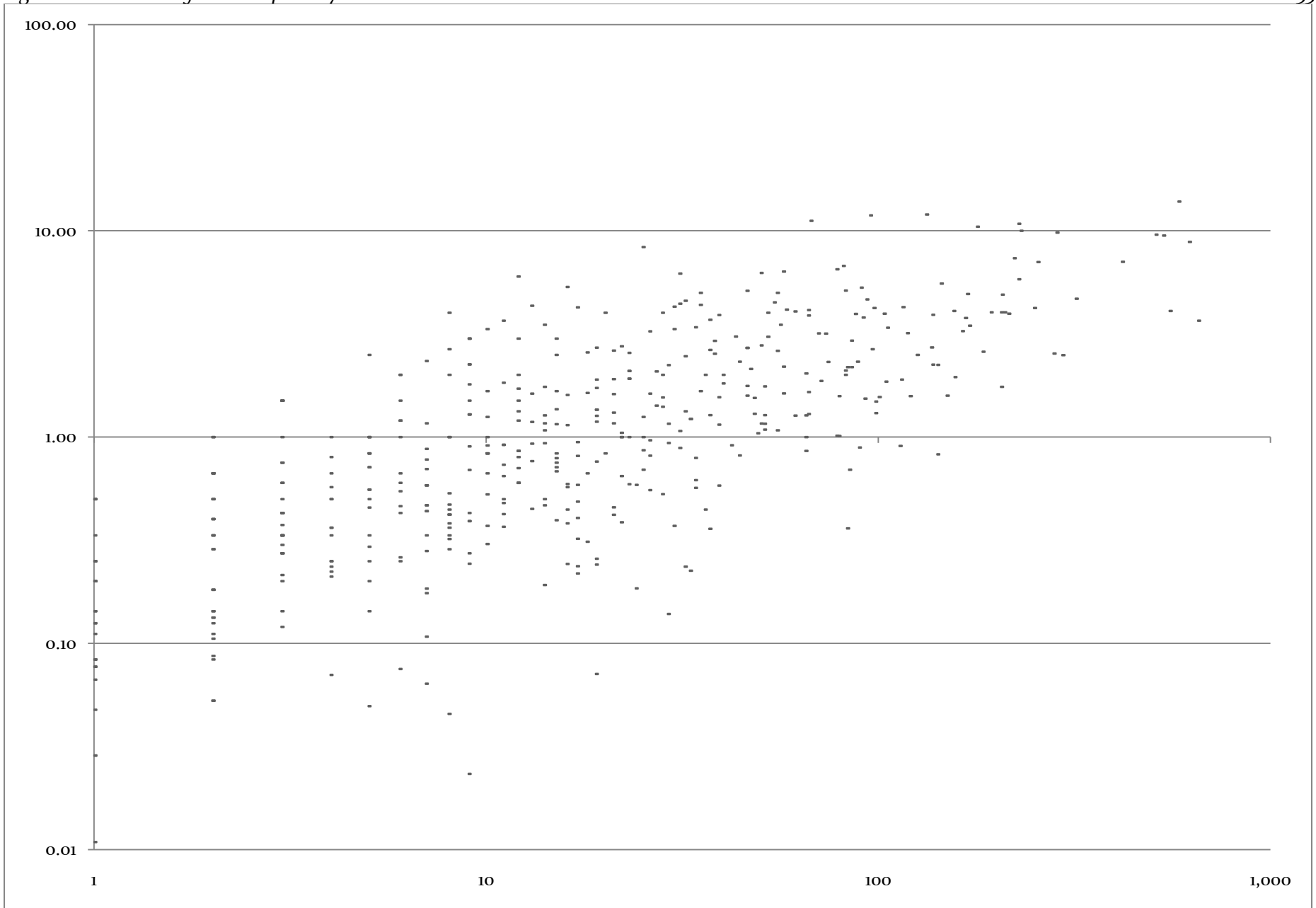
Figure 10.9: Correlation between comment count and CI, 2009
