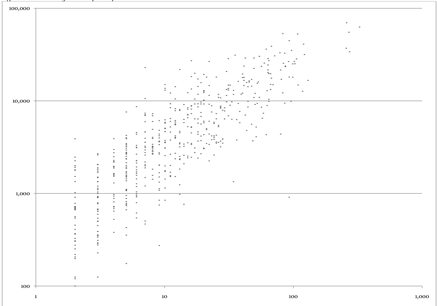
Figure 10.5: Correlation between frequency and total length, 2010
