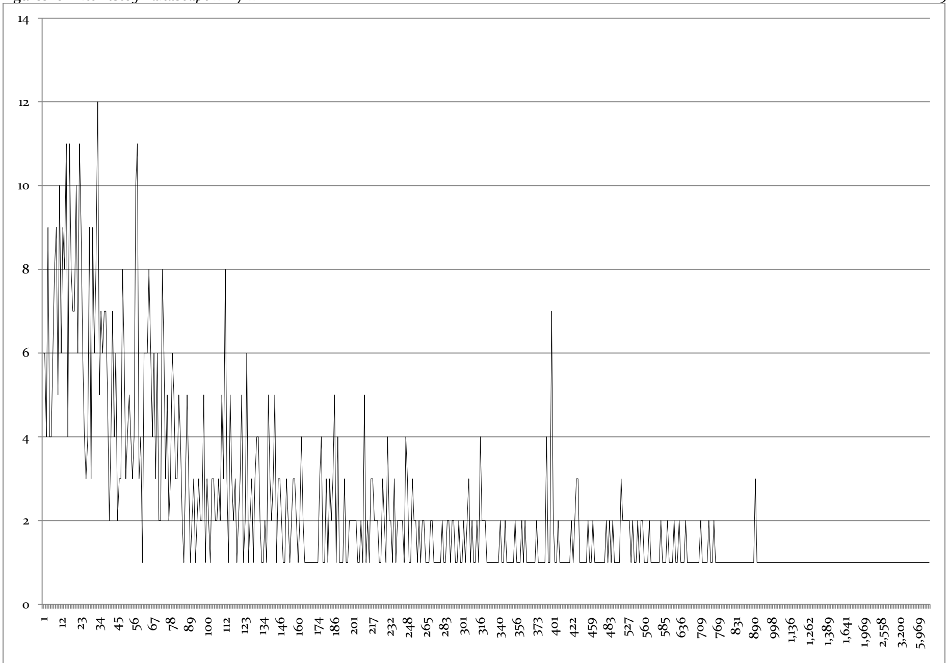
Figure 4.3: Number of blogs for each post total
