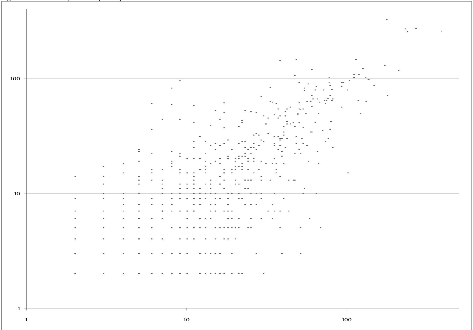
Figure 10.3: Correlation between frequency in 2009 and 2010
