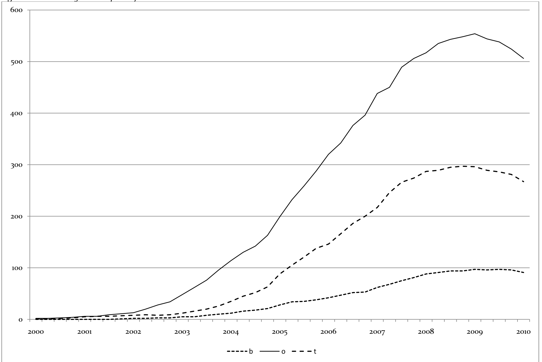
Figure 4.2: Liblogs by type by quarter, February 2000-February 2010
