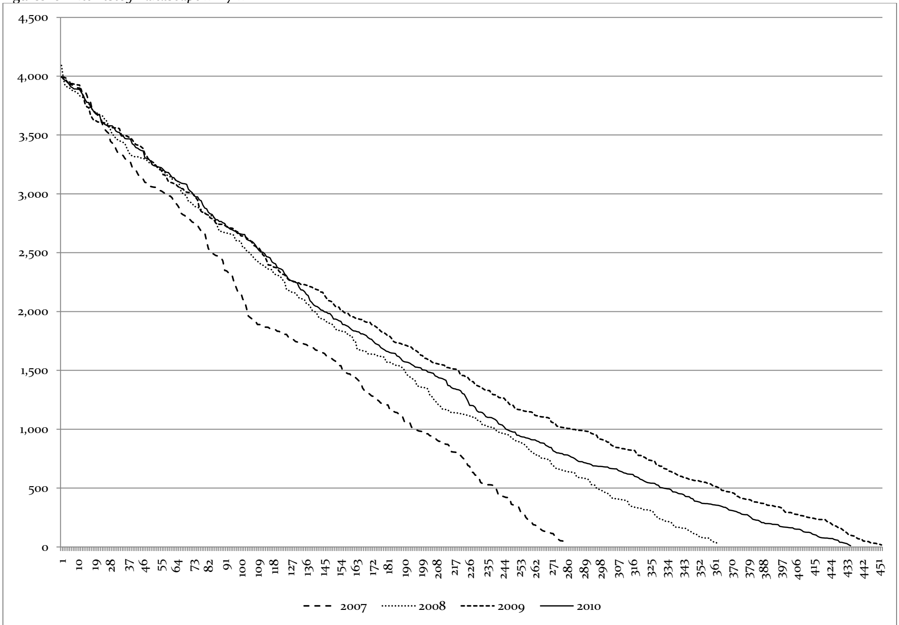
Figure 6.3: Word counts per blog, 11-3,999 words
