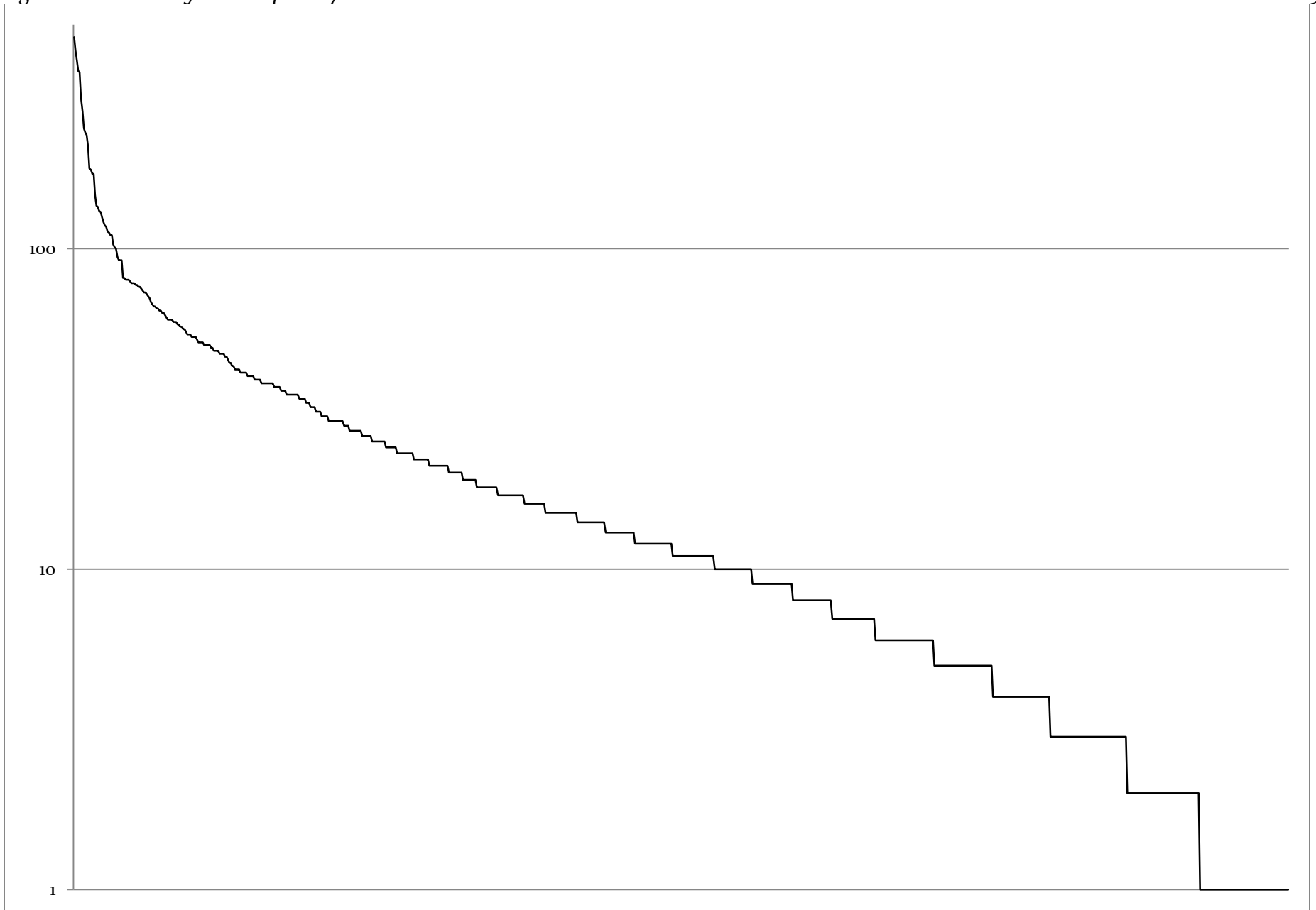
Figure 5.3: Post frequency for March-May 2009
