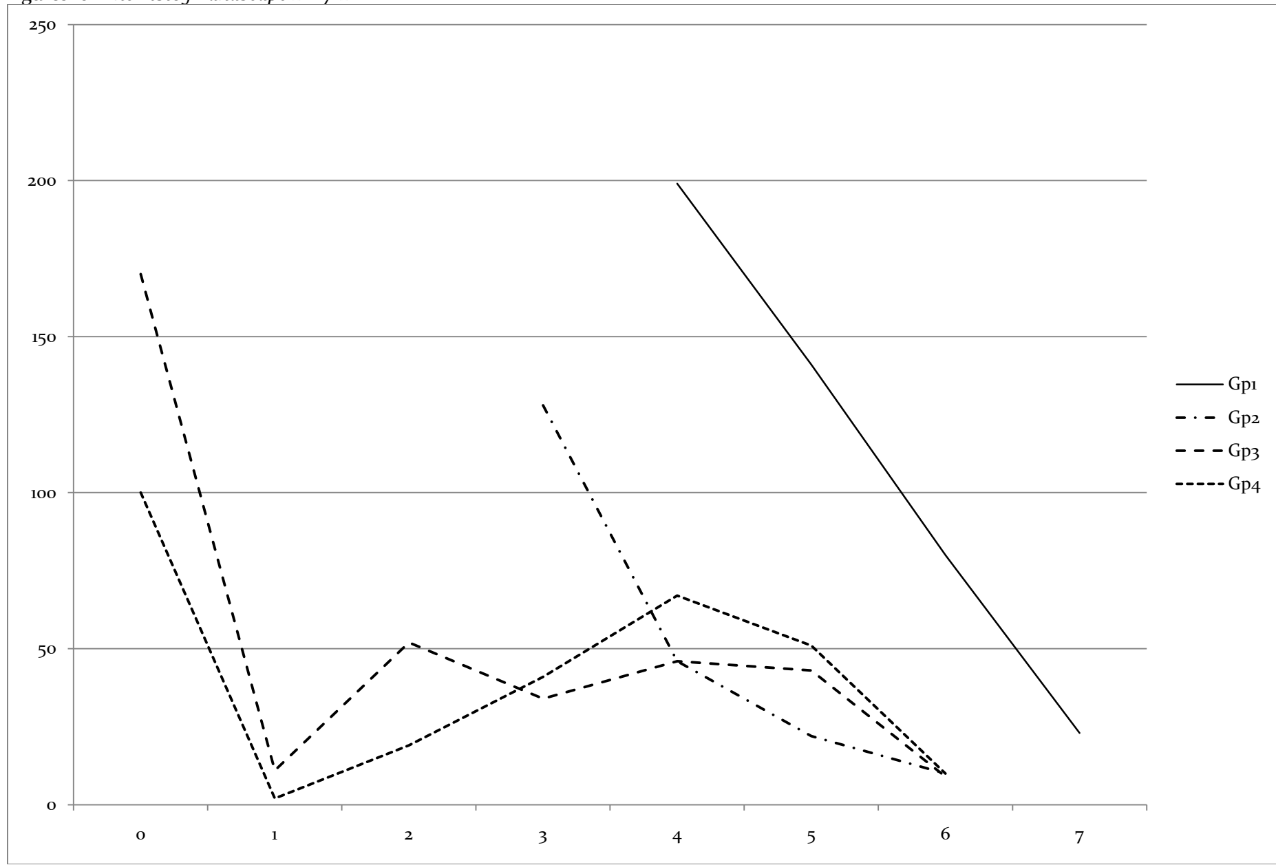
Figure 3.2: GPR for blogs by group
