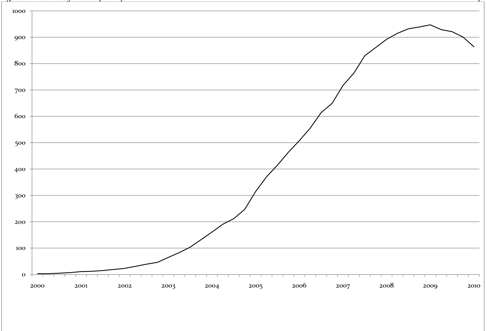
Figure 4.1: Active liblogs by quarter, February 2000-February 2010
