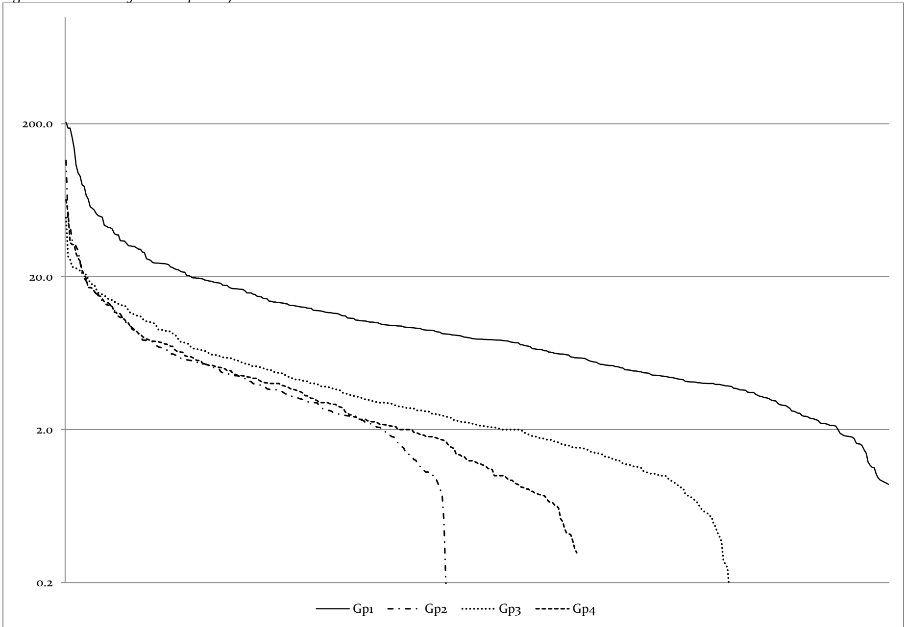
Figure 4.6: Overall post frequency by blog group
