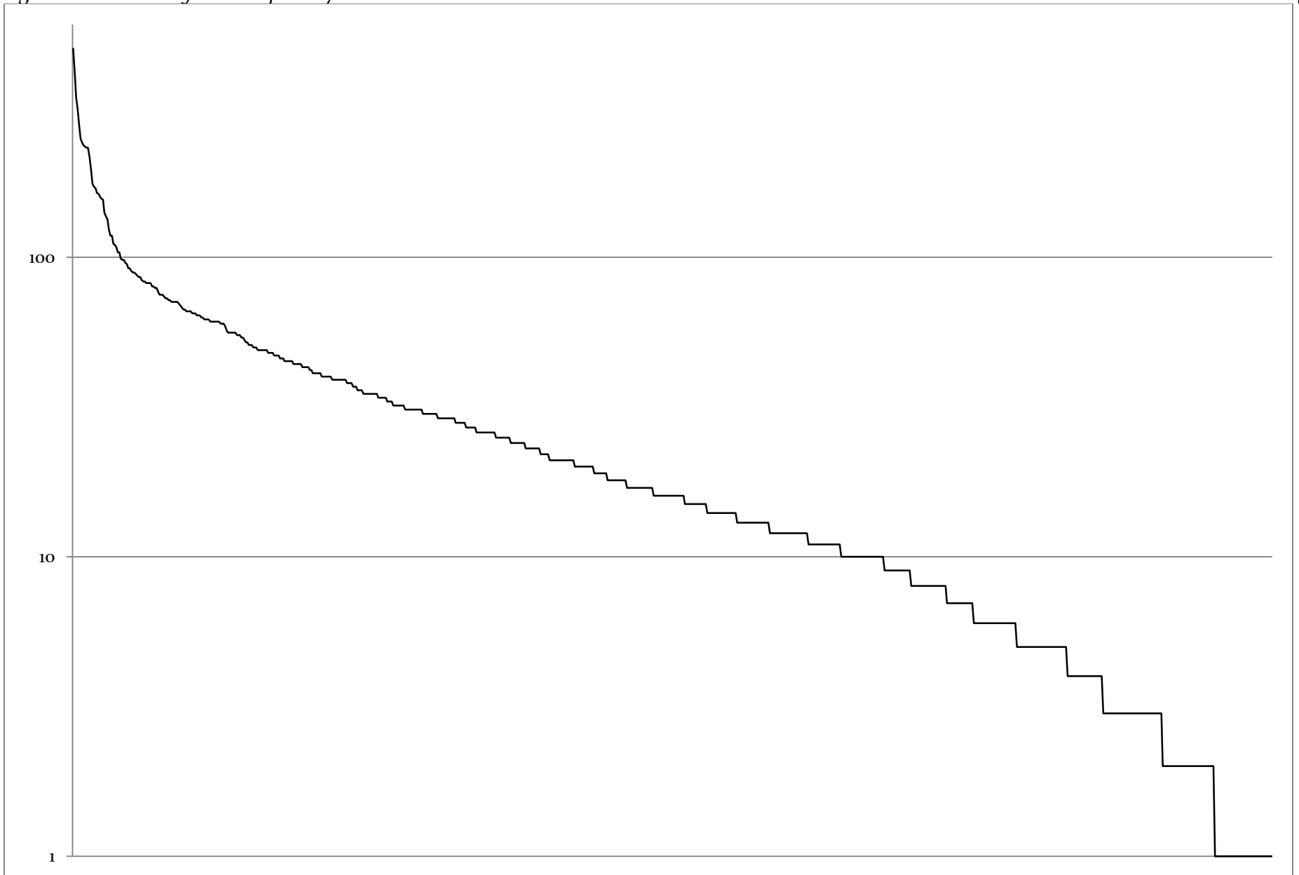
Figure 5.2: Post frequency for March-May 2008
