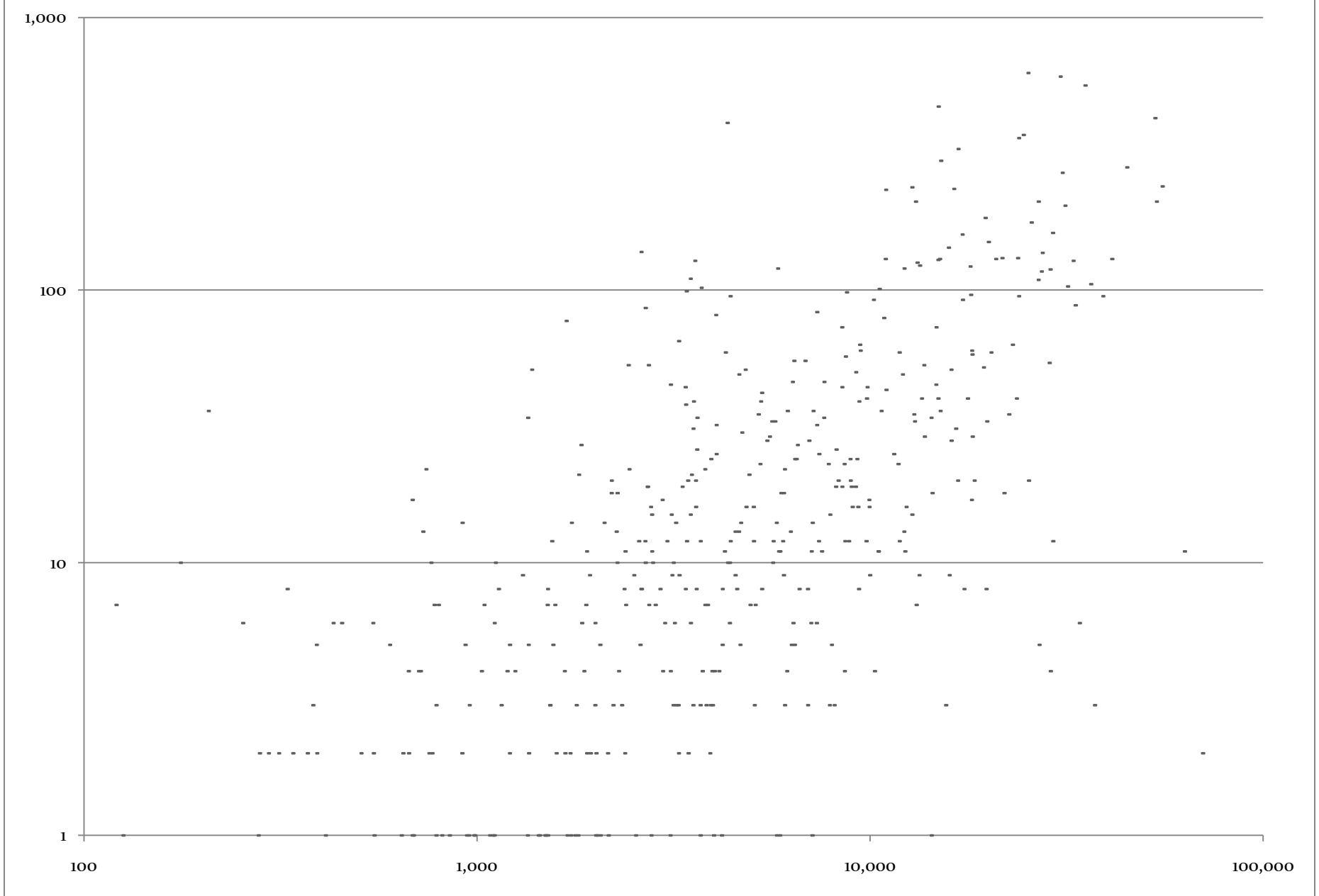
Figure 10.8: Correlation between comments and overall length, 2010
