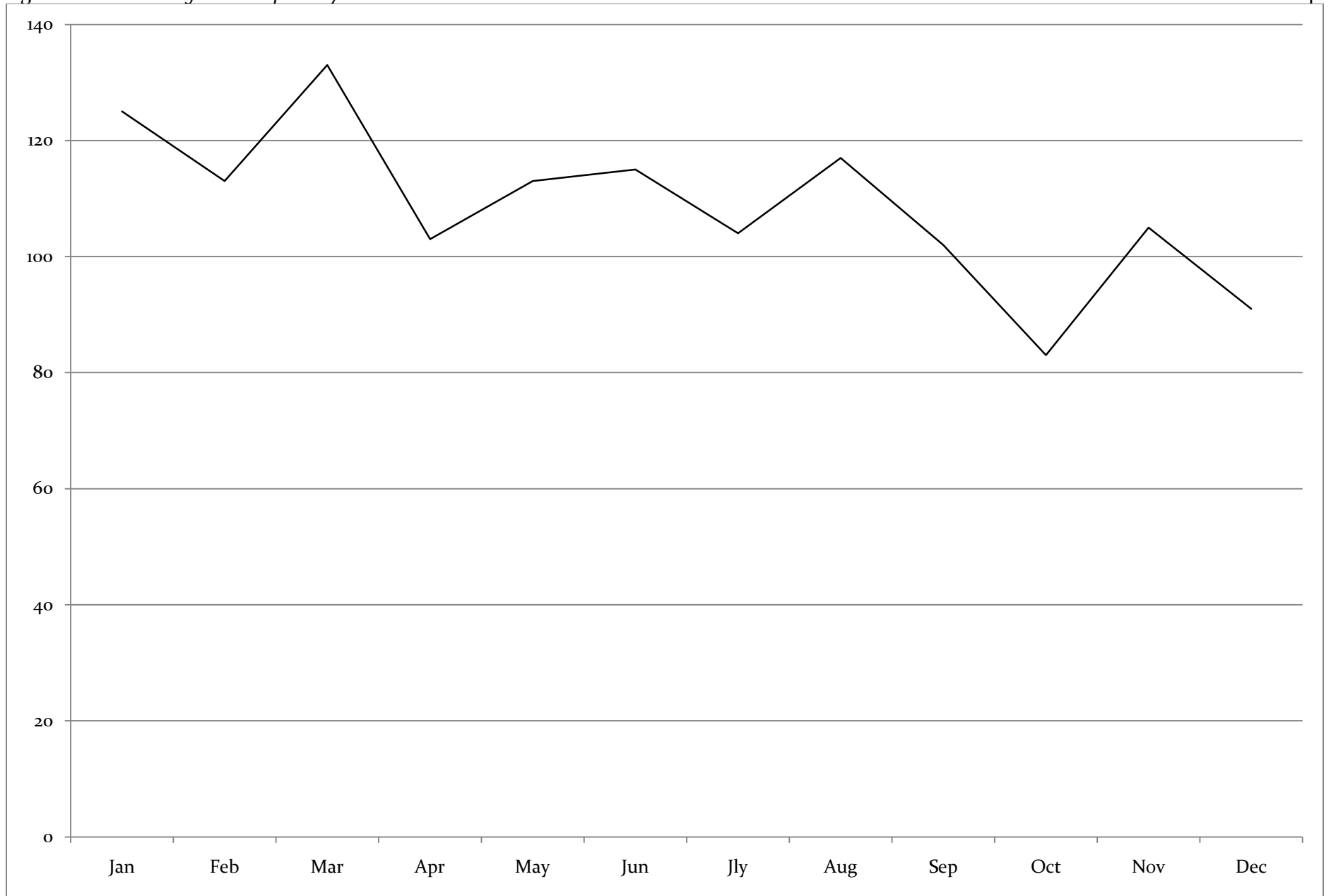
Figure 3.4: Blogs by starting month
