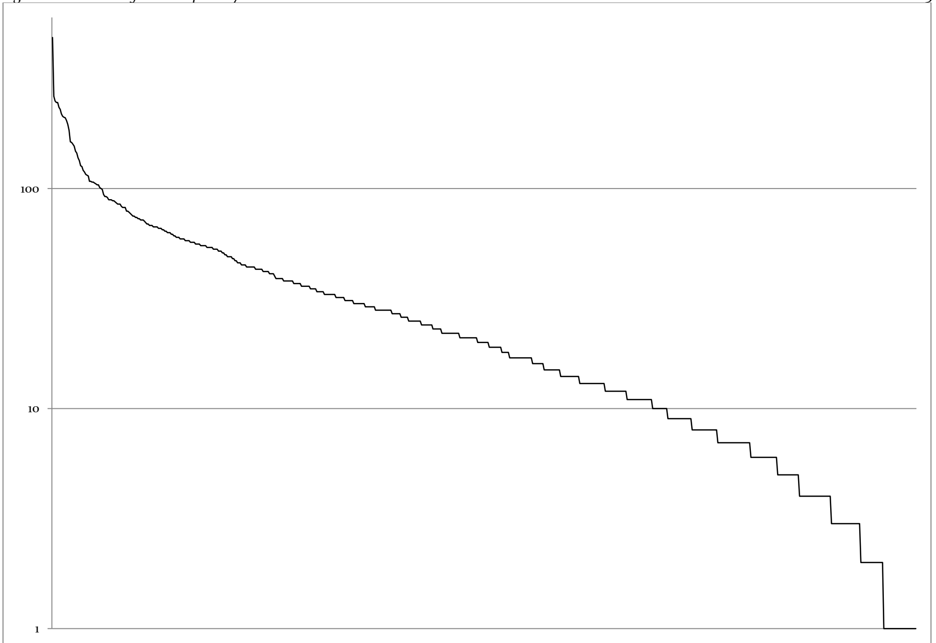
Figure 5.1: Post frequency for March-May 2007
