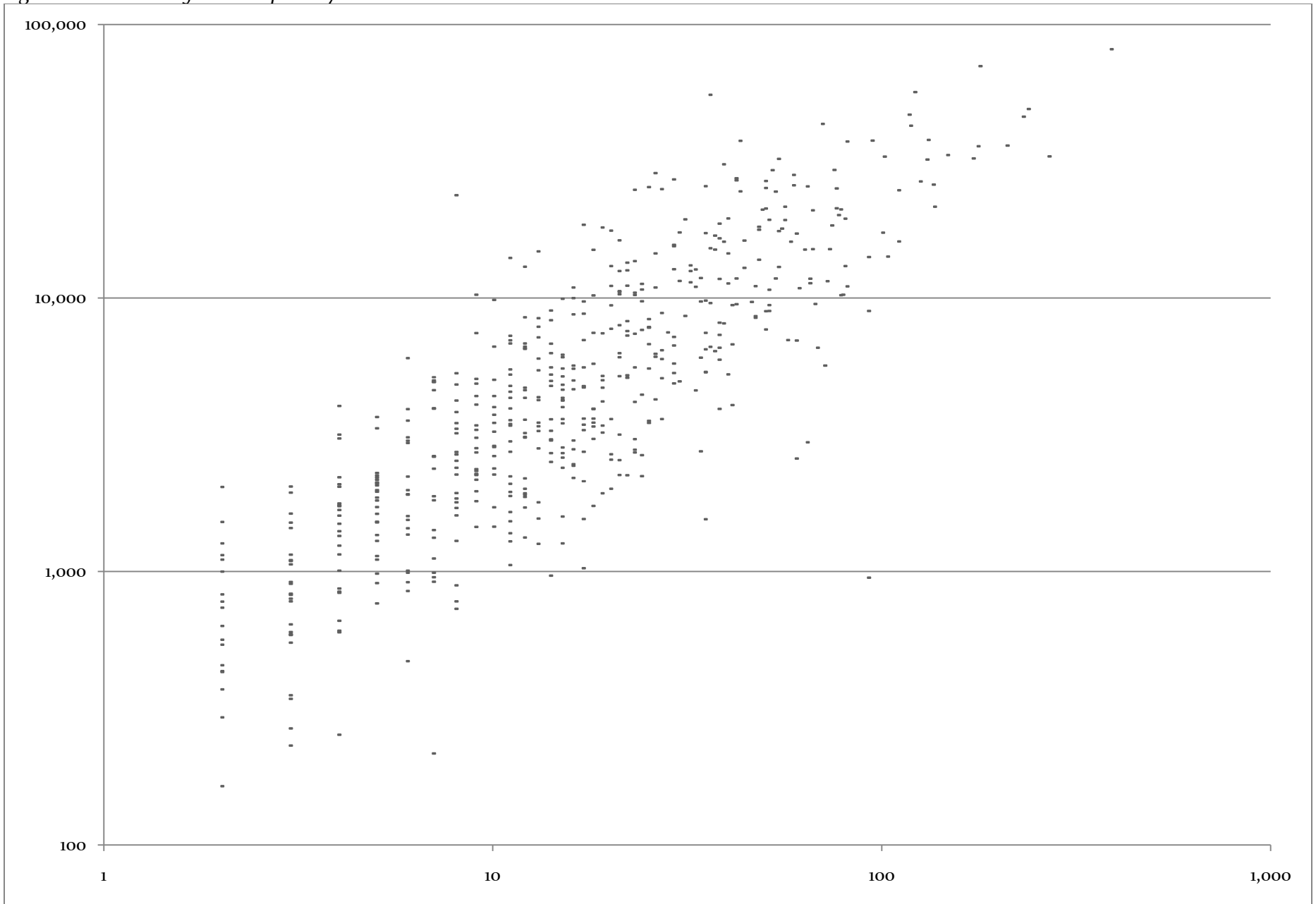
Figure 10.4: Correlation between frequency and total length, 2009
