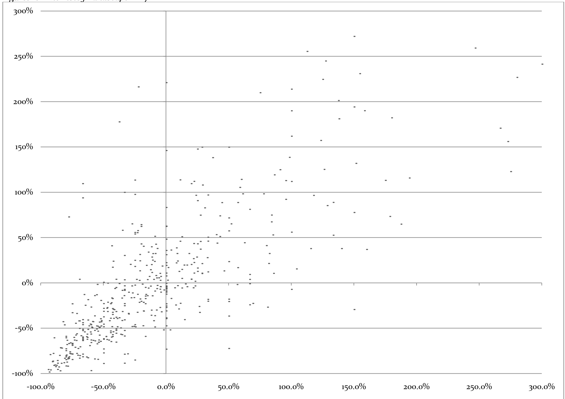
Figure 10.6: Correlation between frequency change and length change
