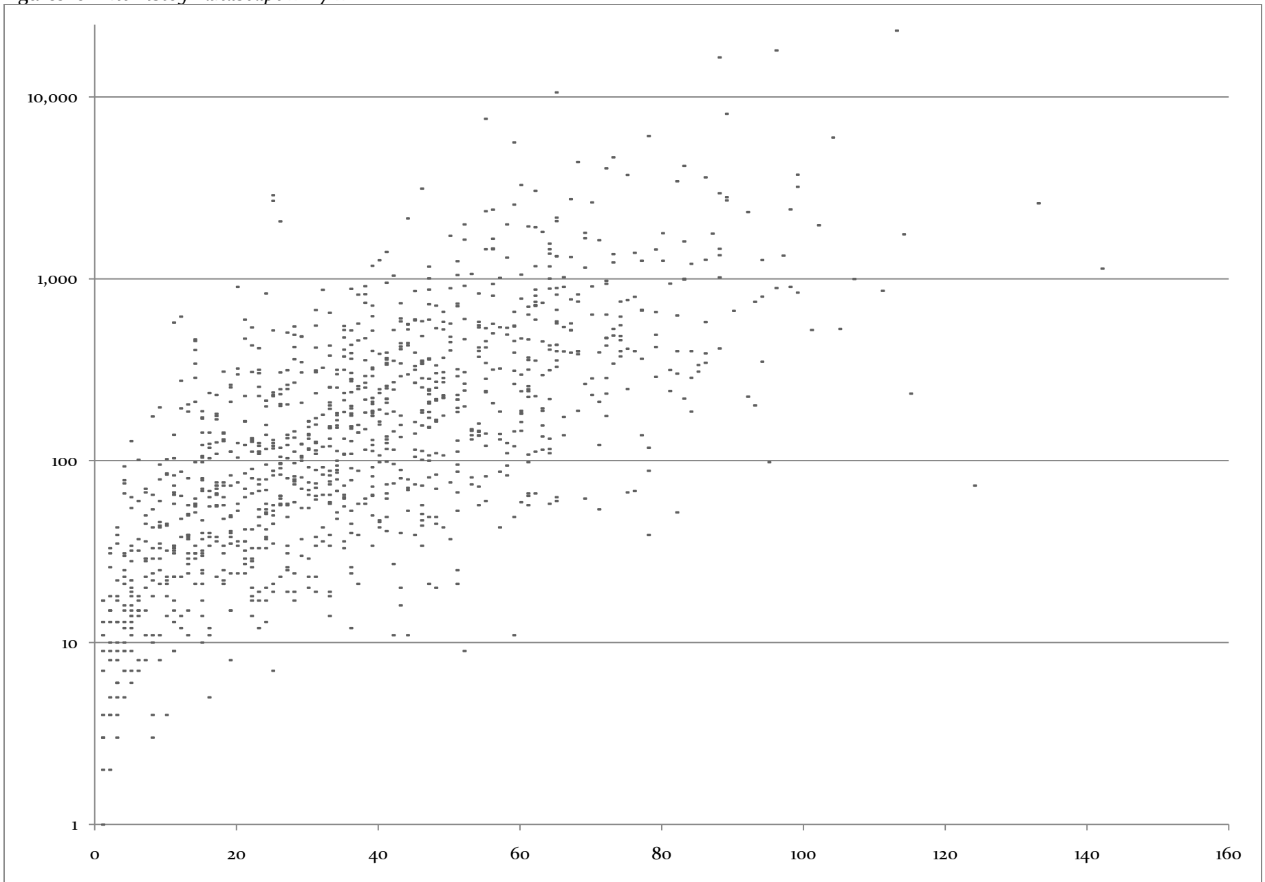
Figure 10.2: Correlation between life of blog and total posts
