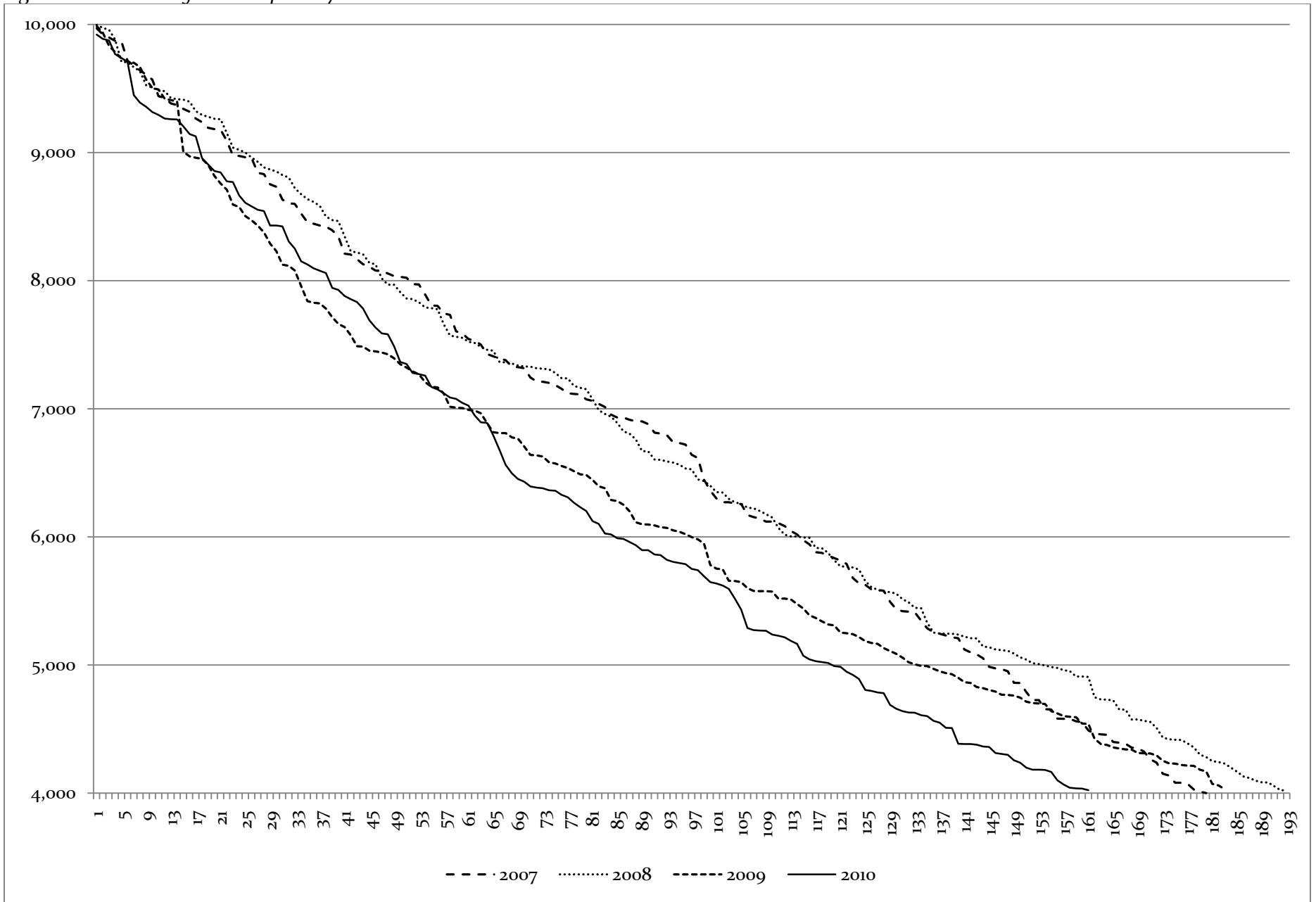
Figure 6.2: Word counts per blog, 4,000 to 9,999 words
