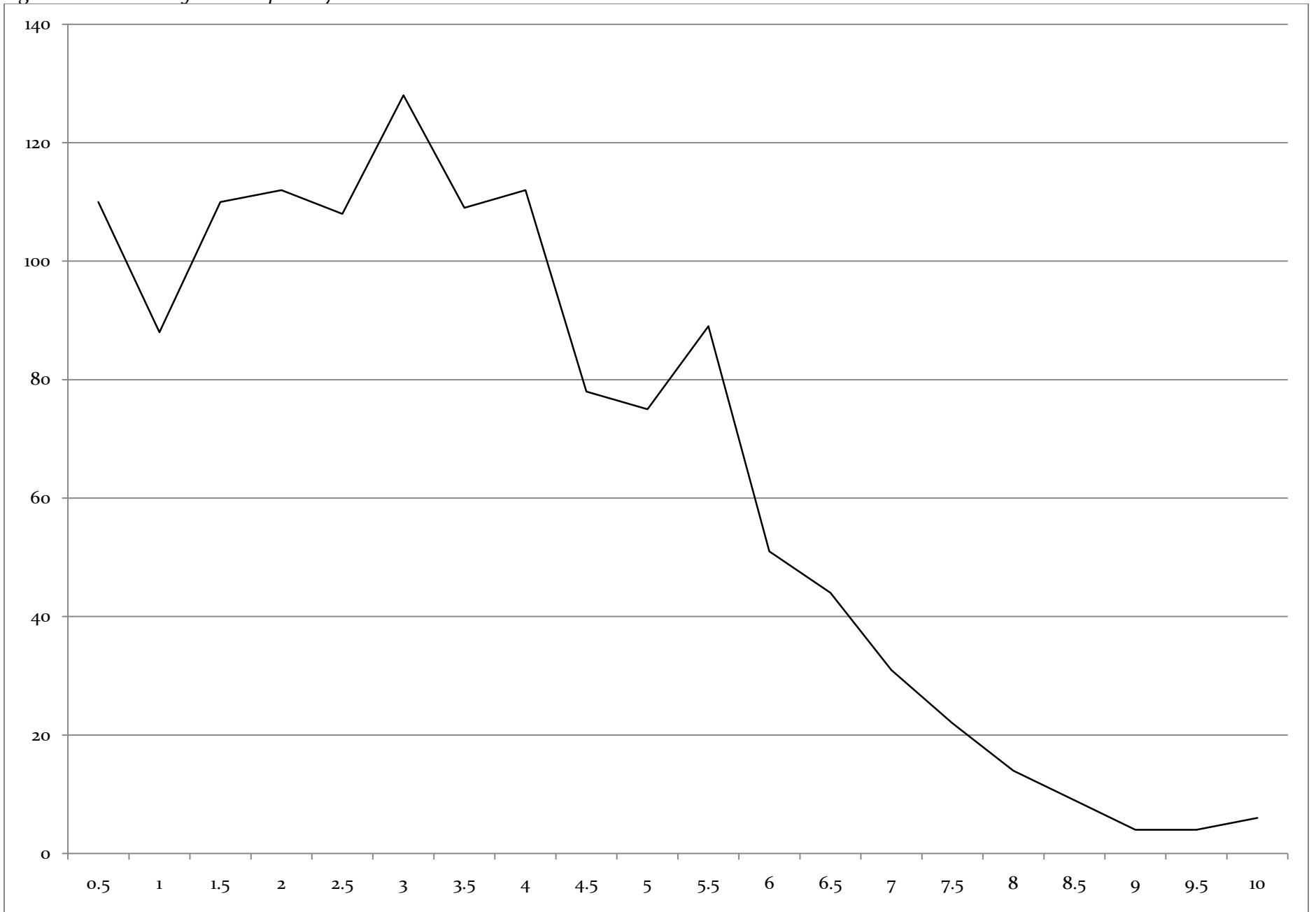
Figure 3.6: Blog longevity by years
