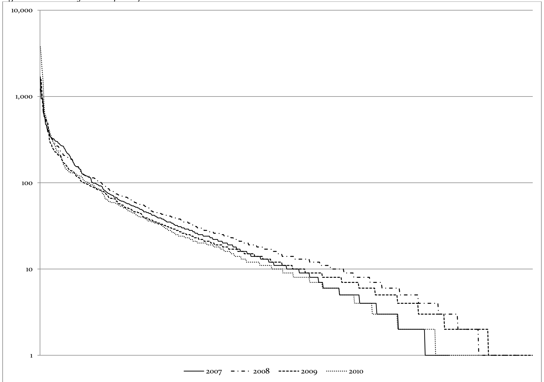
Figure 7.1: Comments per blog, 2007-2010
