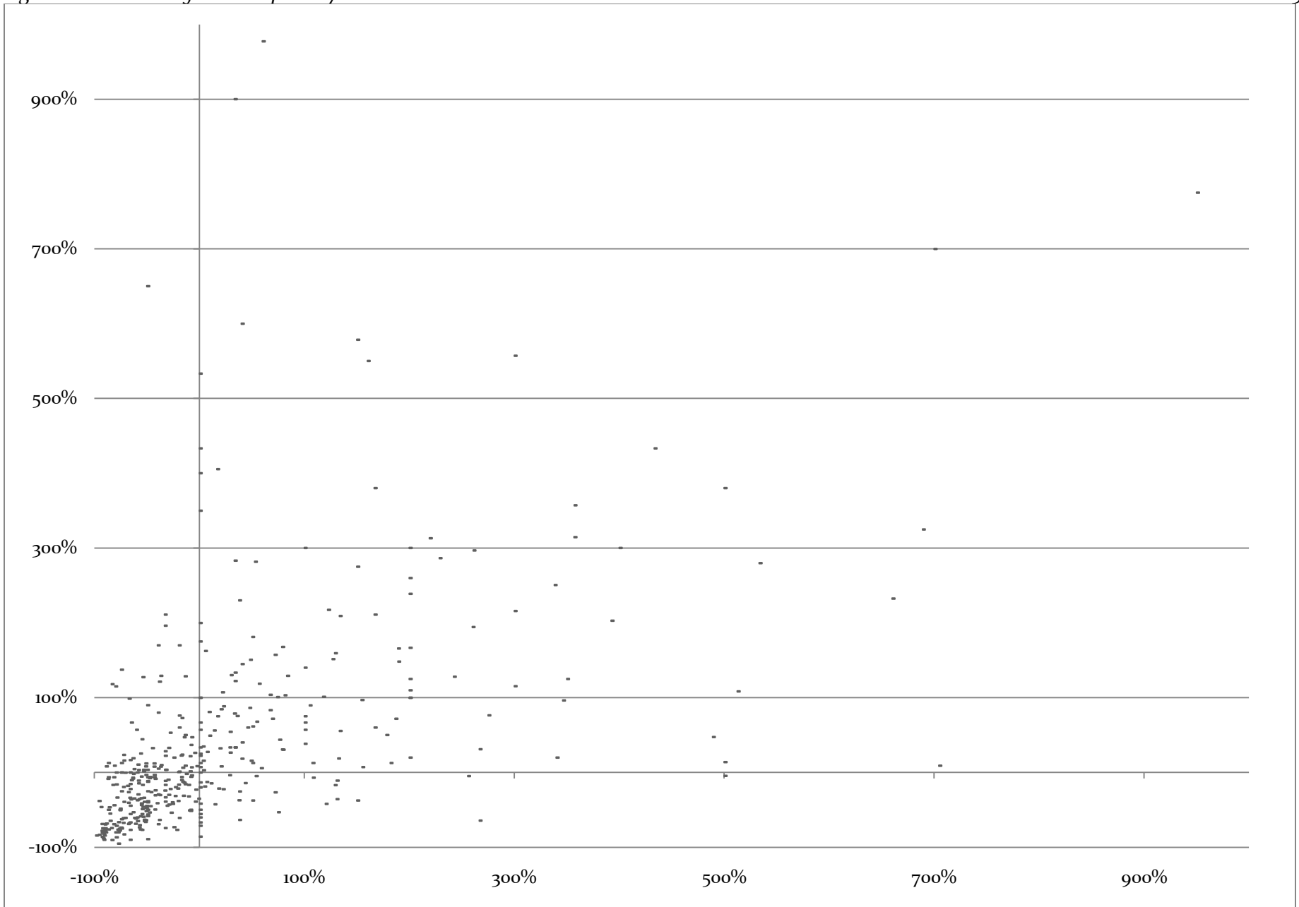
Figure 10.10: Correlation for changes, comments and CI, 2009-2010.
