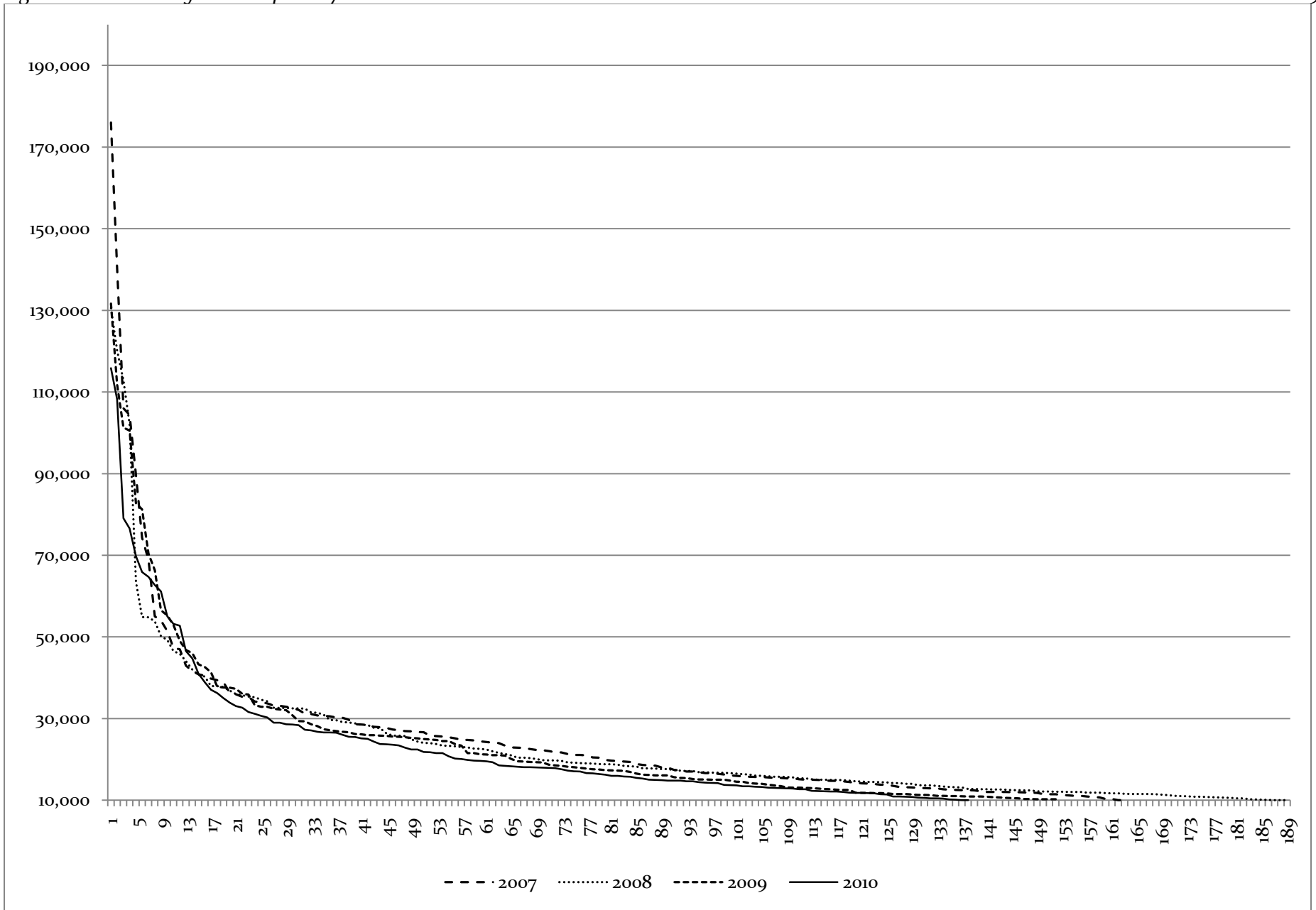
Figure 6.1: Word counts per blog, 10,000 words and up.
