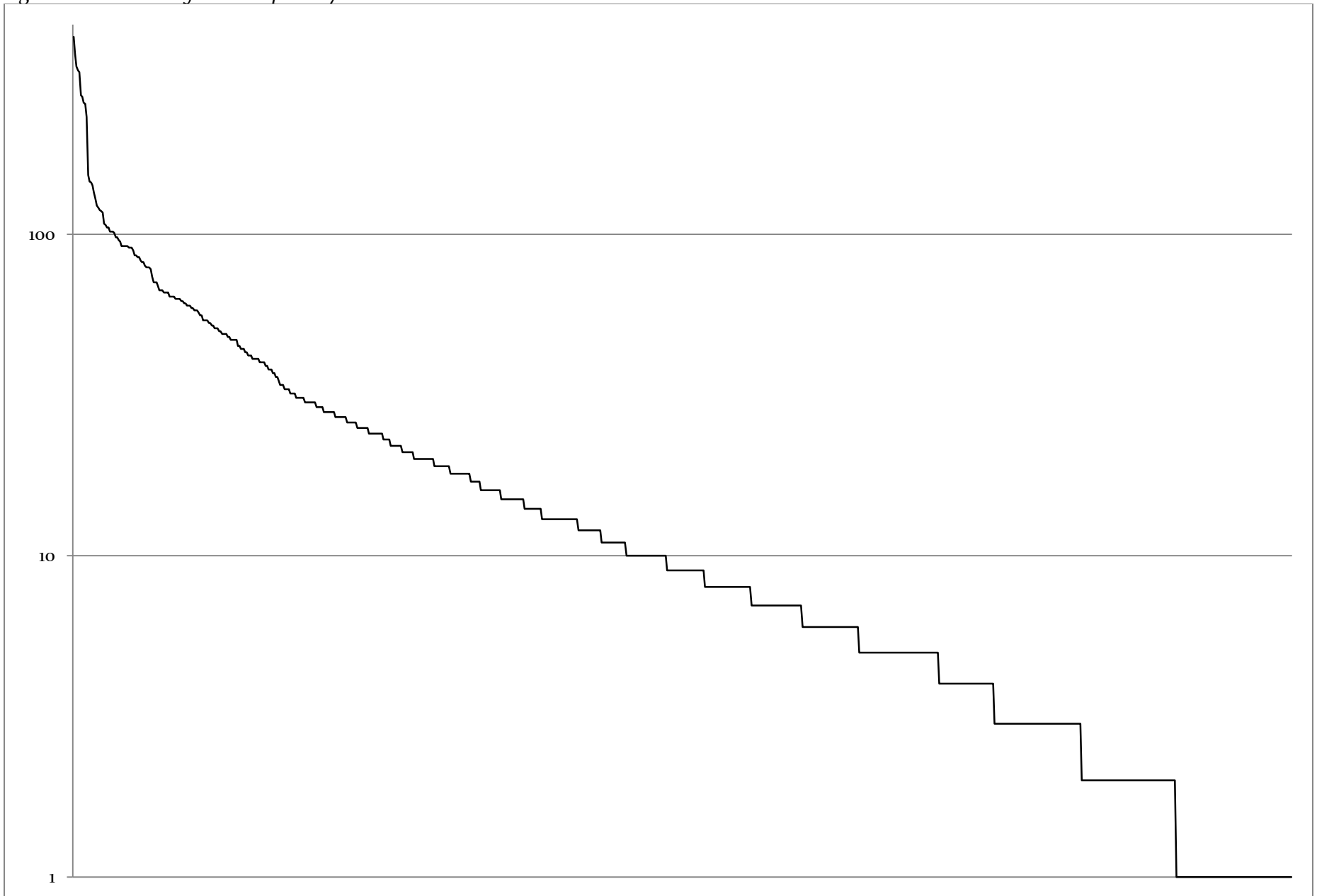
Figure 5.4: Post frequency for March-May 2010
