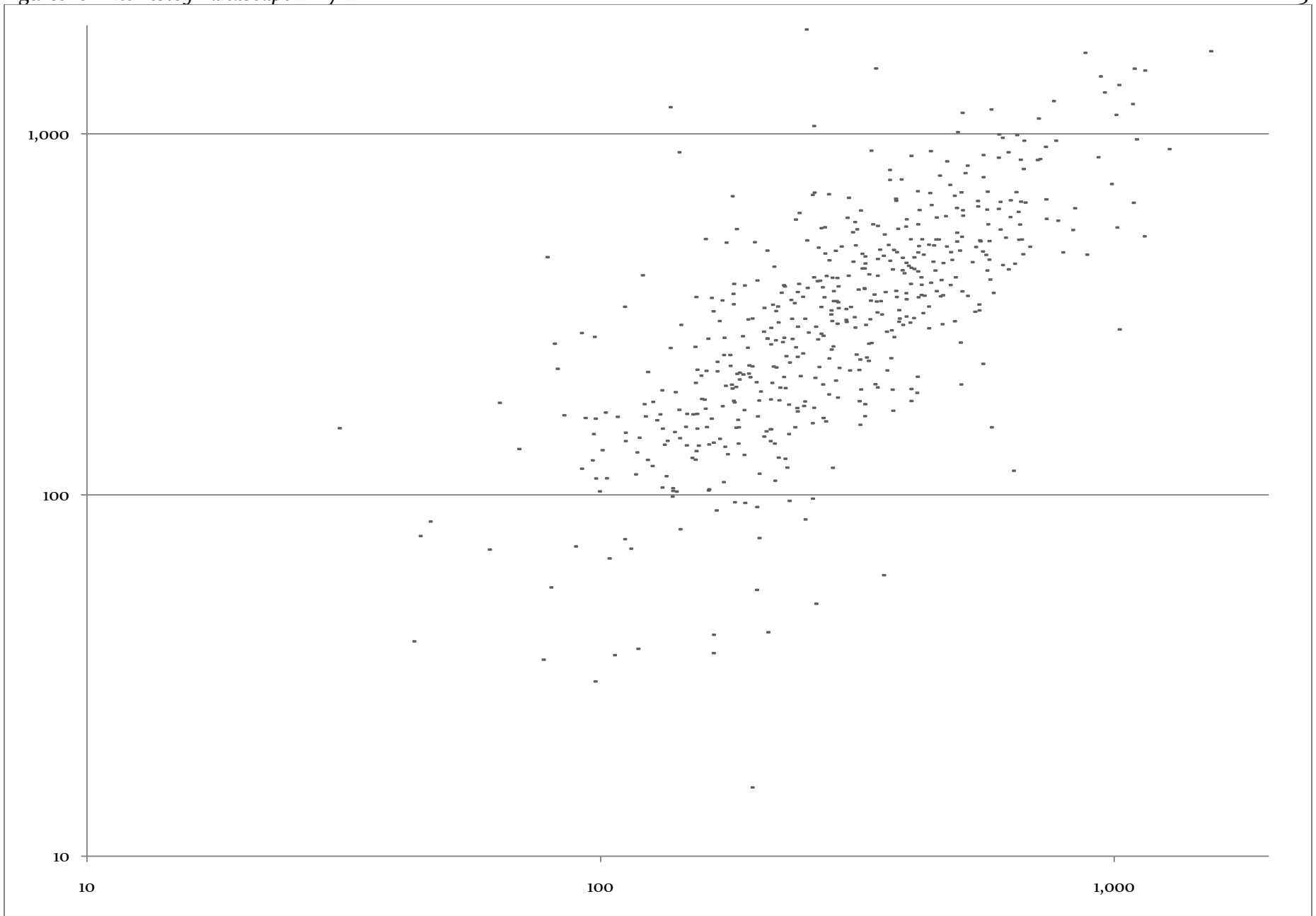
Figure 10.7: Correlation between words per post in 2009 and 2010
