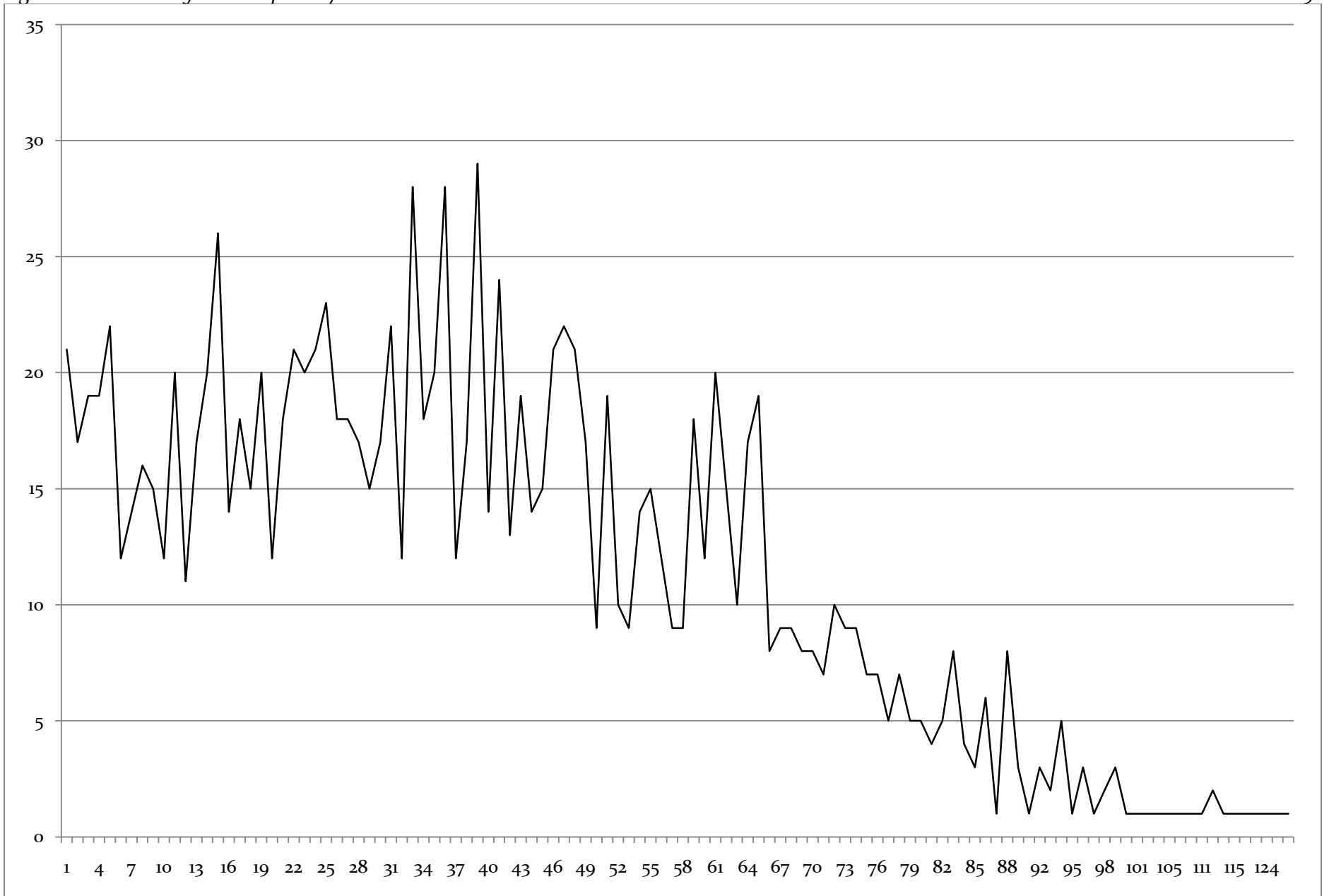
Figure 3.5: Blog longevity by months
