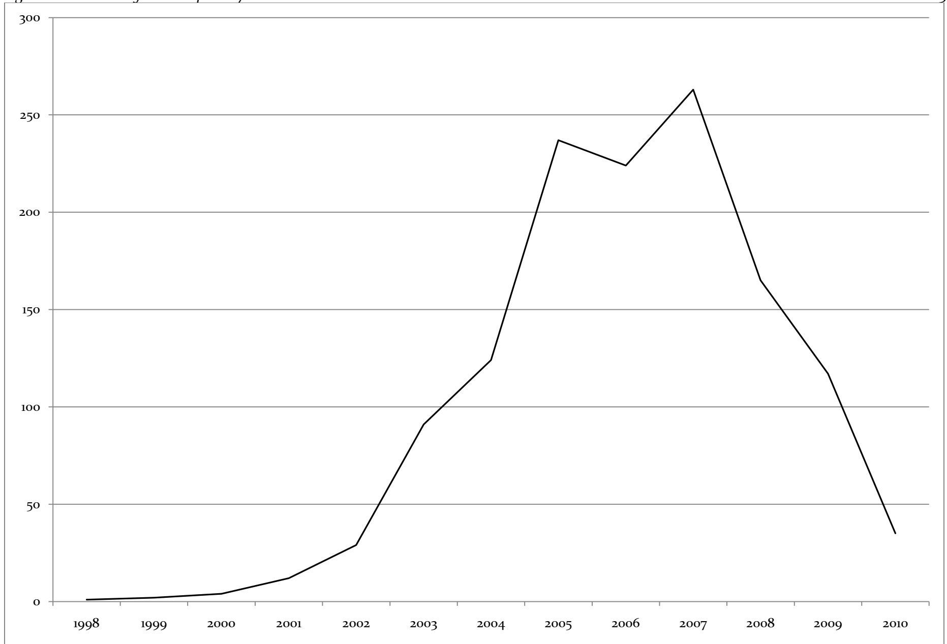
Figure 3.3: Blogs by starting year
