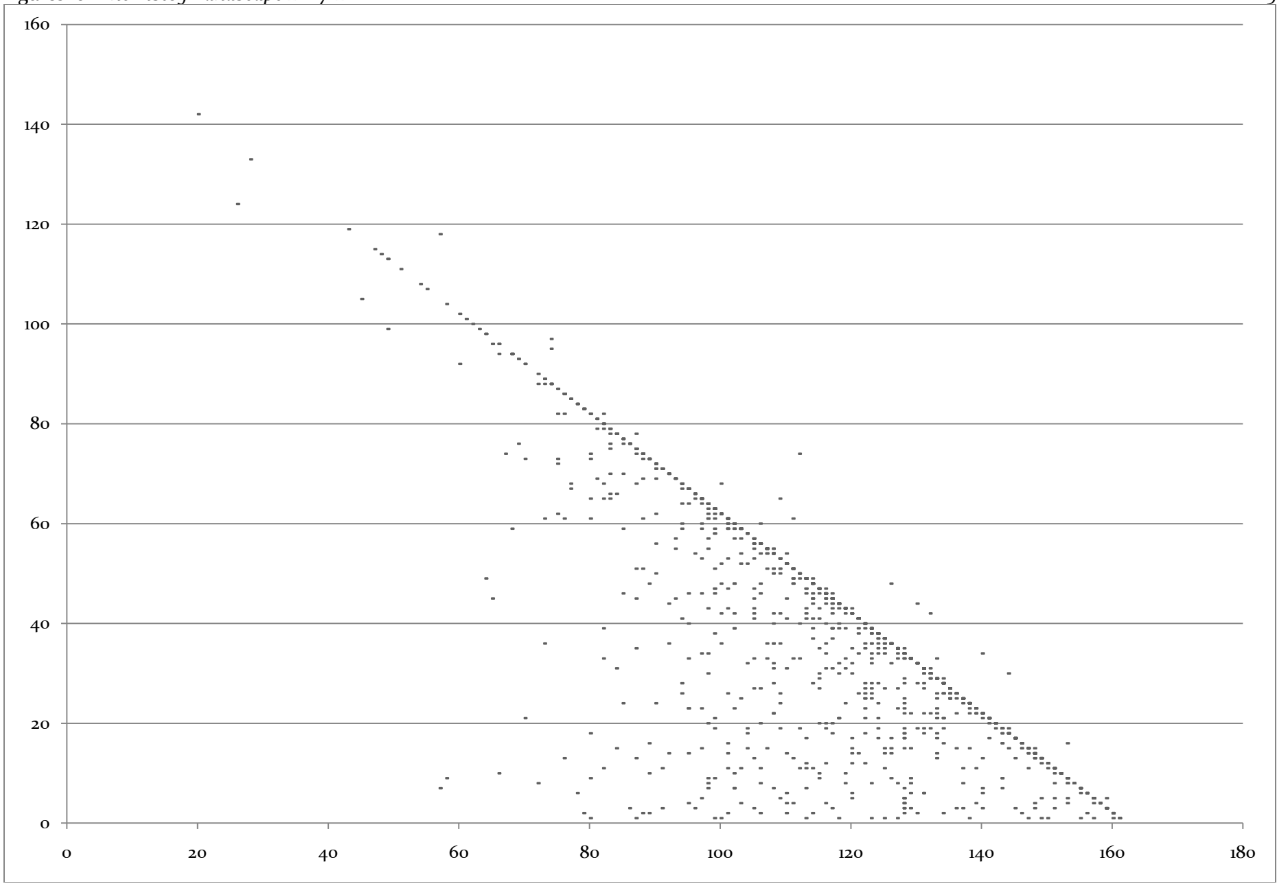
Figure 10.1: Correlation between start of blog and life of blog
